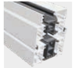
STEPPED sash, FLUSH frame
