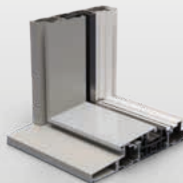
Standard outer frame with clip-on cill nose
